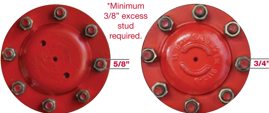
5/8" Axle Bolts
